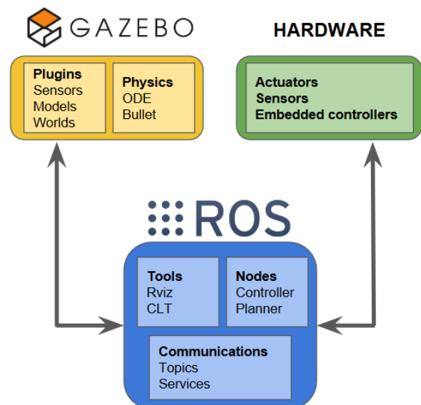
Fig. 1: Diagram visualizing the correlation between ROS, GAZEBO and the robot hardware to be simulated, whereas the pluggable design of ROS allows for easily substituting a real world system without having to change the controlling algorithms [2].
