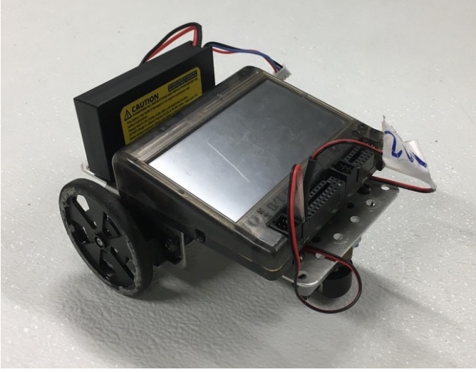
Fig. 4: For experimental purposes, a relatively simply built robot was used, consisting of a metal base plate, two solarbotics wheels powered by standard Botball® motors, a ball-caster wheel and the KIPR Wallaby.
