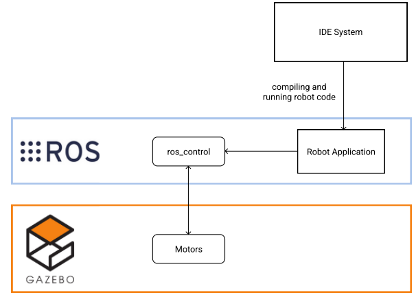
Fig. 3: Diagram depicting the architecture of ARIS.
